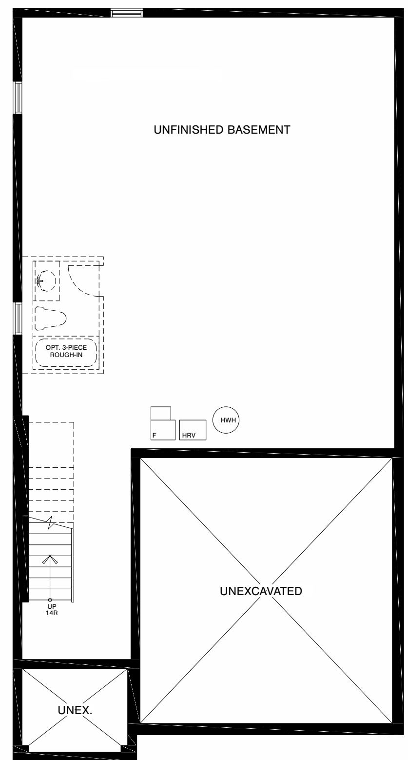
Basement
