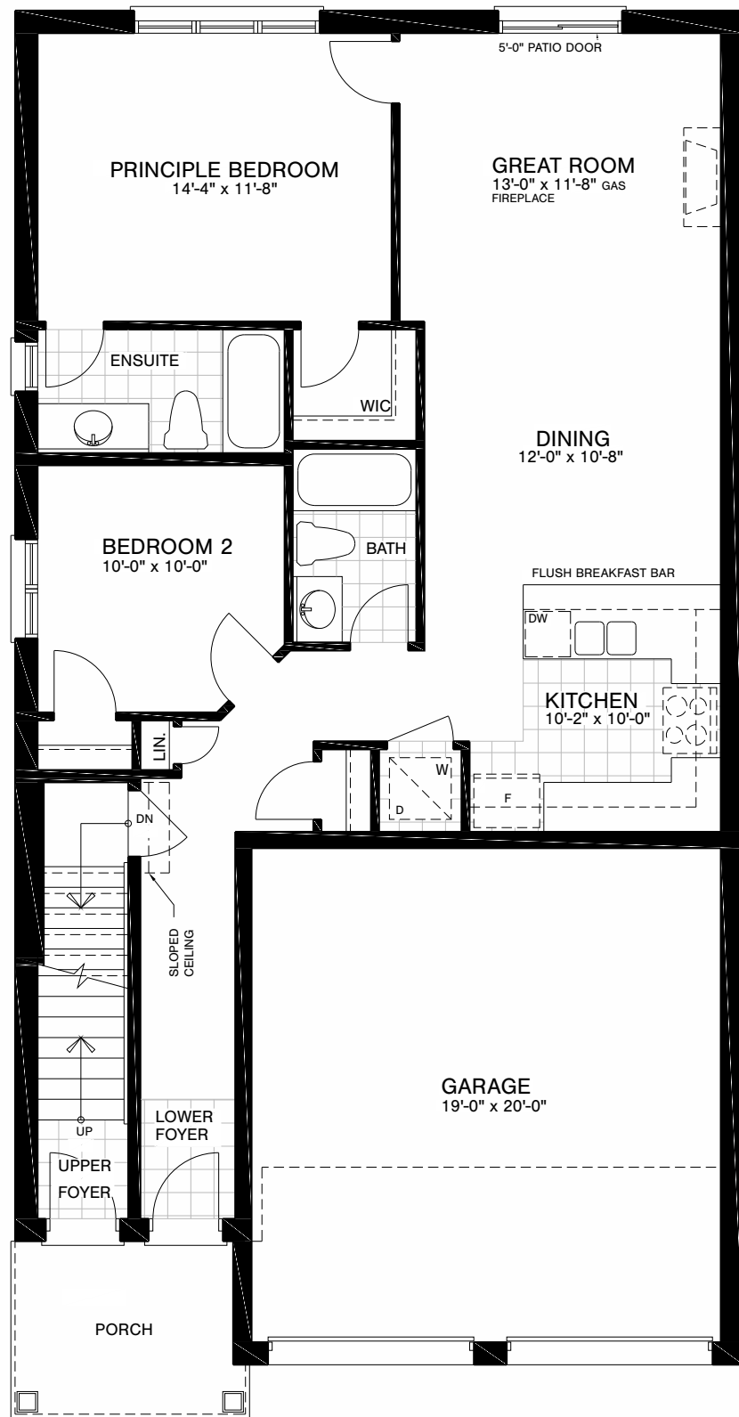
Ground Floor
